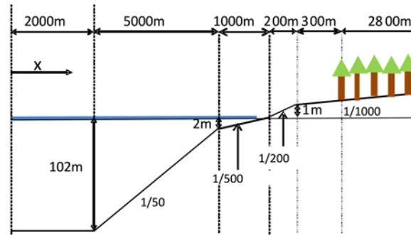
Fig. 11 Beach topography model (Case-1)
